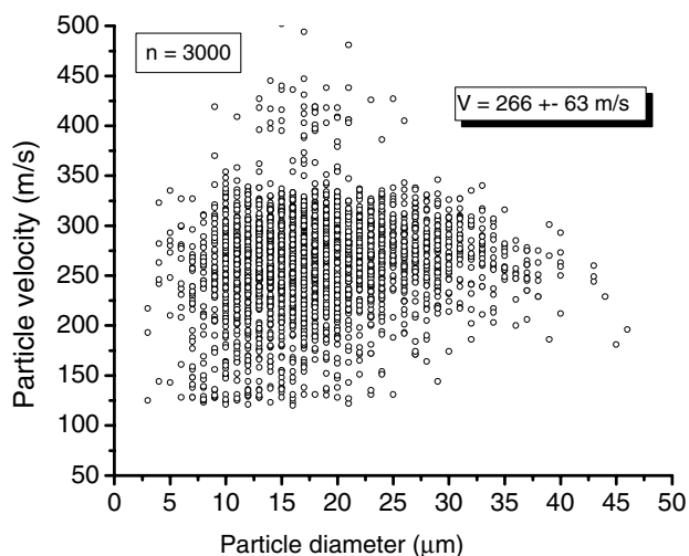
Fig. 2. Particle velocity versus particle diameter distribution in the plasma jet.
